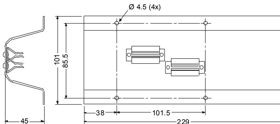
Fig. 8 Outdoor shield
