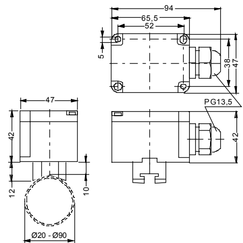
Fig 4 Strap-on Sensor
