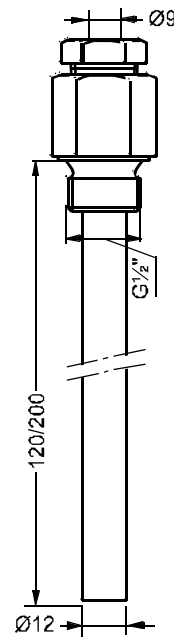
Fig. 10 Stainless steel wells TS-9100-891x
