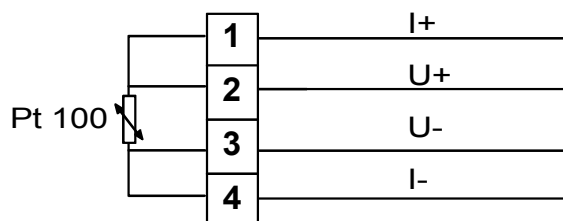
Wiring diagrams Pt-100 models
