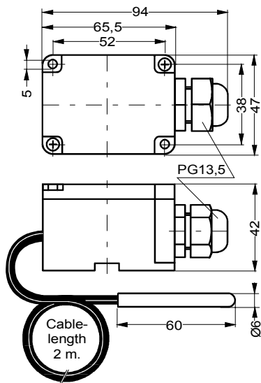
Remote sensor TS-9101-810x
