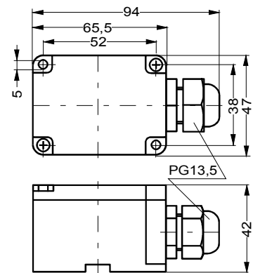
Outdoor sensor TS-910x-840x
